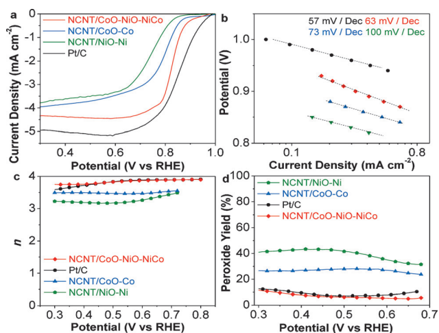
Figure 3. a) ORR polarization curves of NCNT/CoO-NiO-NiCo, reference catalysts, and Pt/C (Scanning rate: 10 mVs -1 , rotating rate: 1600 rpm, the loading is 0.21 mg cm -2 ). b) The Tafel plots of NCNT/CoO-NiO-NiCo, reference catalysts, and Pt/C. c) The electron transfer number n of NCNT/CoO-NiO-NiCo, reference catalysts, and Pt/C at different potentials. d) Percentage of peroxide with respect to the total oxygen reduction products.
